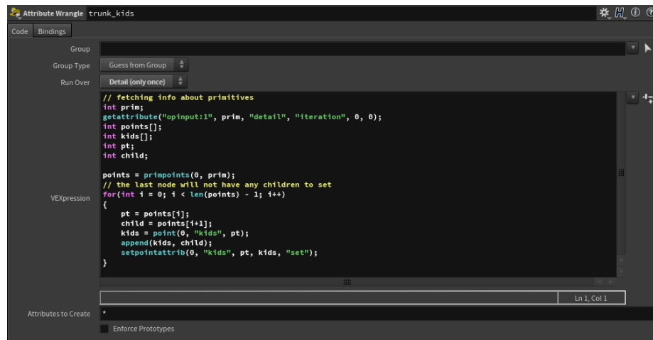
Figure 4: Wrangle node interface
