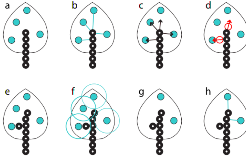
Figure 3: Space Colonization Algorithm by Runions et al (2007)
