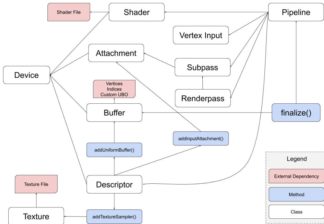
Figure 4.12: vulkan architecture.
